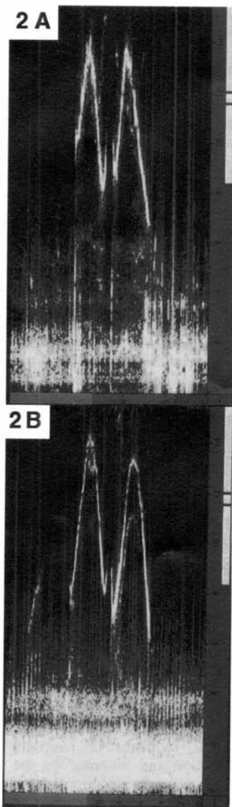
Figures 2-8. Spectrograms of signature whistles for individual dolphins of varying age class and sex. Many of the listed individuals have whistles that have been visually scanned, over ten years, for consistency but have not been captured electronically. Therefore, a minimum number ( n ) of captured whistles, and repetitive years (yrs) during which whistles were recorded are given. Frequency is on the vertical and time on the horizontal axis for all figures.
