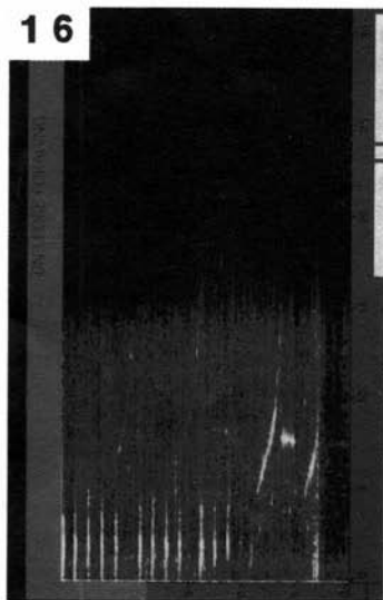
Figure 16. Spectrogram of trills, and upswept whistles during ledge feeding by bottlenose dolphins.
