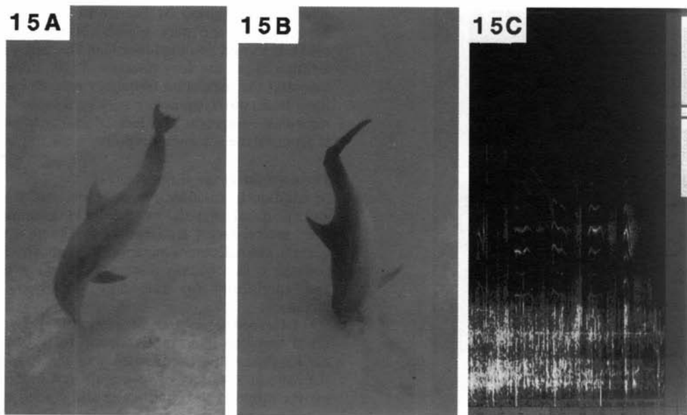
Figure 15. Foraging behavior—bottlenose dolphins. (a and b) Bottlenose dolphin orients and penetrates sand with rostrum; (c) spectrogram of razor buzz during penetration into sand with rostrum. (Clicks appear harmonic in nature due to the high repetition rate of >500 clicks per second [Watkins, 1967].)
