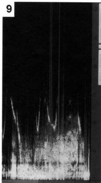
Figure 9. Spectrograms of an excitement vocalization of juvenile dolphin.
